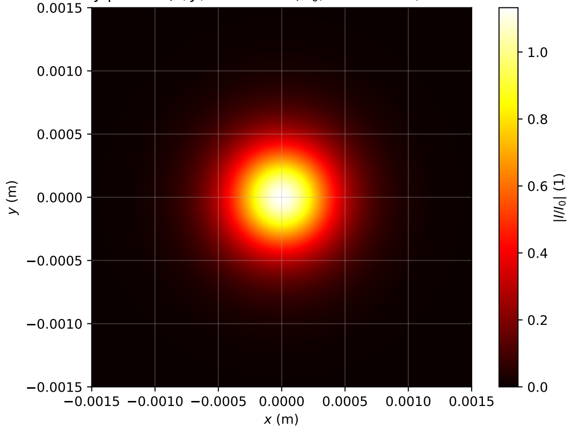
Intensity profile I(x, y, z = 2.866m)/I_0 , P_{in}=0.8P_{cr} , artificial time
